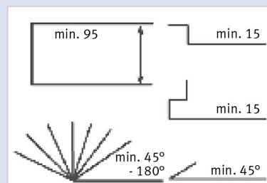
Bending examples HSBM with low and high top beam
